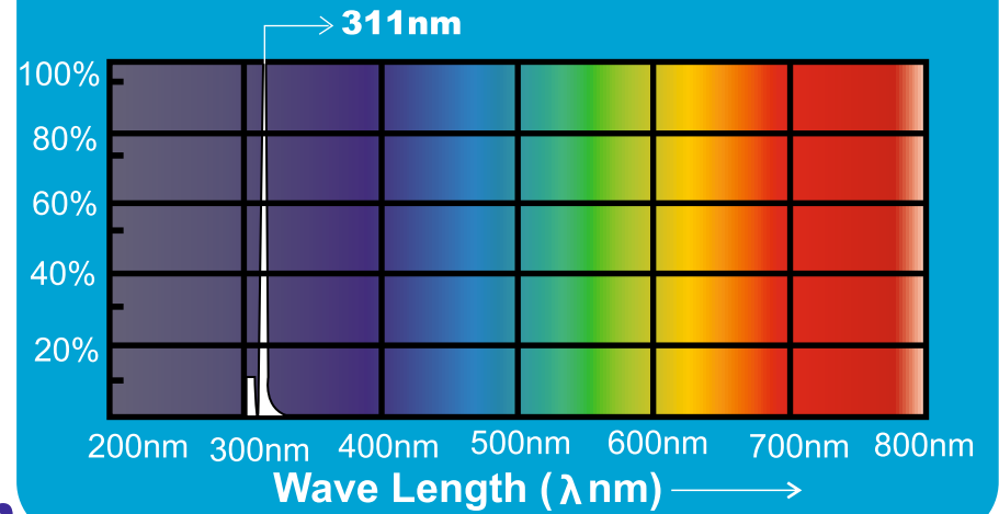
PHOTOMETRIC RESPONSE OF NBUVB DEVICE:
